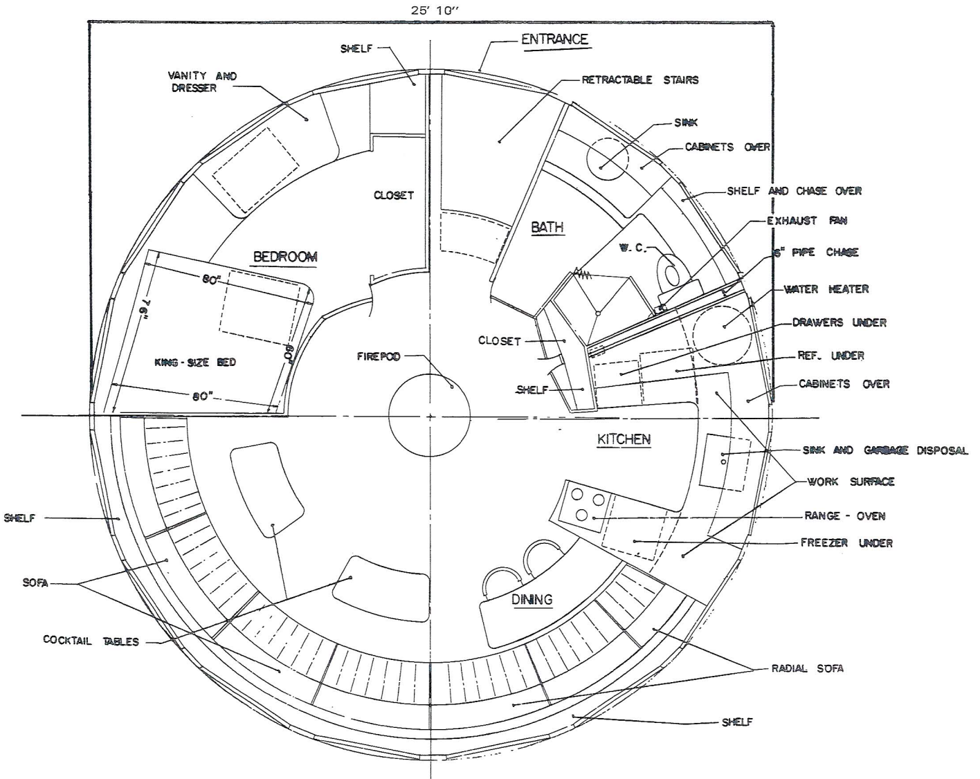
FLOOR PLAN
